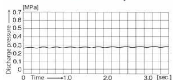
With Pulsation Dampeners
