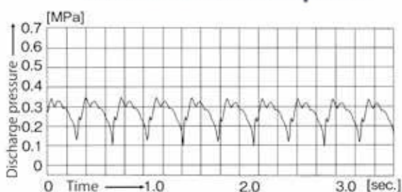
Without Pulsation Dampeners
