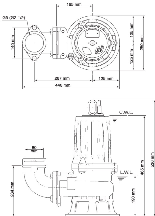
C.W.L. = Continuous running water level 80B21.5-52 (A-11452-1) L.W.L. = Lowest running water level
