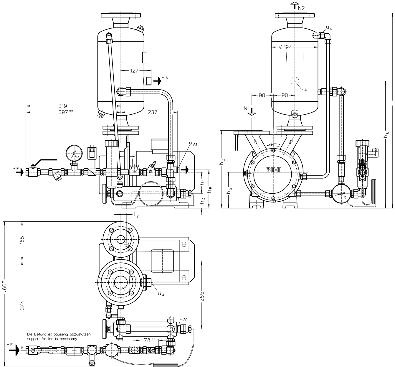
Arrangement drawing LEM 91, 126, 161 with thermostatic control
